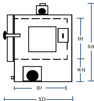
SIDE VIEW (w/Doors)
