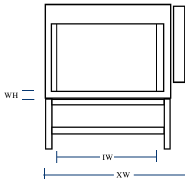
FRONT VIEW (wo/Doors)
