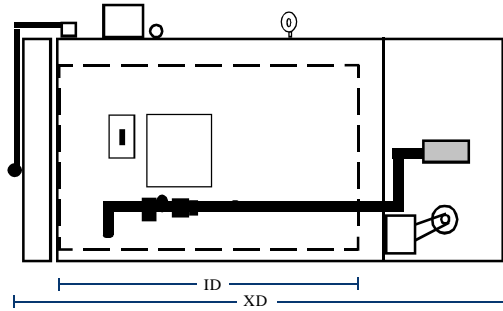
SIDE VIEW (w/ Doors)
